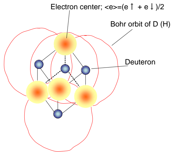
Fig. 4: Electron orbits of TSC at t = 0 , namely orthogonally coupled state of two \text{D}_2 molecules as transient motion, with life time about 40 to 80 fs.
