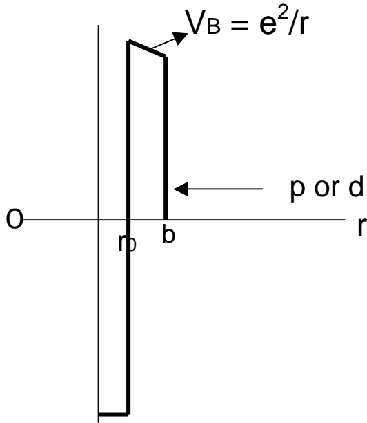
Figure 5: Potential for Coulomb barrier penetration and strong negative well, for Sudden Tall Thin Barrier Approximation (STTBA)
