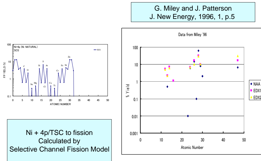
Fig.7: Fission products by Ni + 4p/TSC reaction, calculated by SCS model 13) and experimental data by Miley-Patterson 7)
