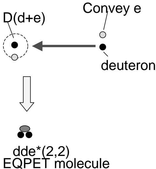
Fig.1: Formation of dde^*(2,2) molecule by d-beam injection into condensed matter
