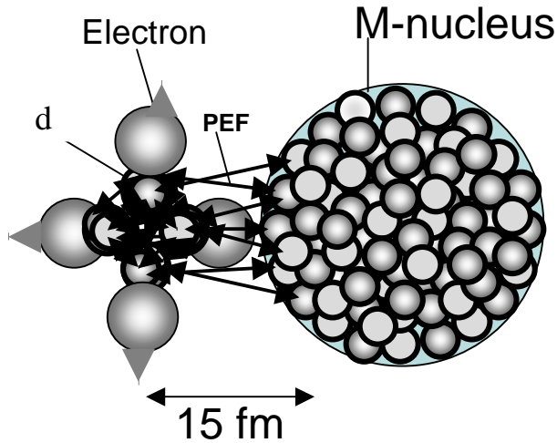
Fig.6-b): Strong interaction for 4d/TSC + M-nucleus
