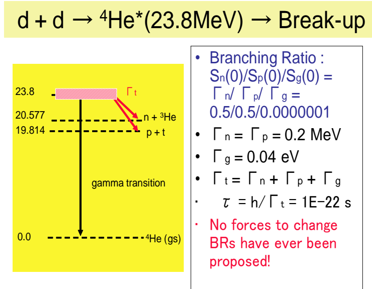
Fig. A-1: Break-up channels of d-d fusion reaction
