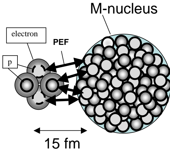
Fig.6-a): Strong interaction for M-nucleus + 4p/TSC
