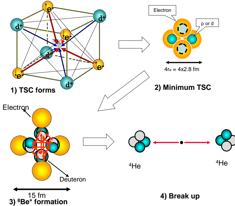
Fig.3: Semi-classical view of squeezing motion of TSC, \langle e \rangle = (e \downarrow + e \uparrow)/2 for QM view at 4 electron centers.
