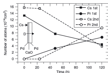
Fig. 7. Variation of Cs and Pr concentration
