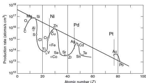
Fig. 3 Reaction product yield vs. Atomic number (Miley)
