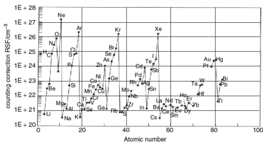
Fig. 4 Yield of elements formed on Pd surface (Mizuno)
