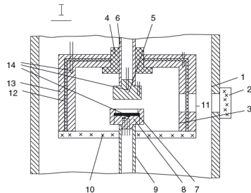
Fig. 1 Glow Discharge apparatus used by Karabut et al.
