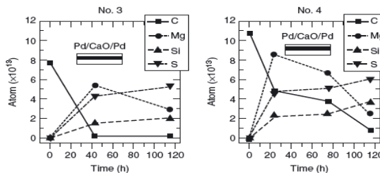
Fig. 6 XPS measurement of time dependence of C, Mg, Si, and S on surface of multilayer Pd samples
