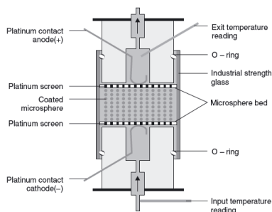
Fig. 2 Schematic of Patterson power cell
