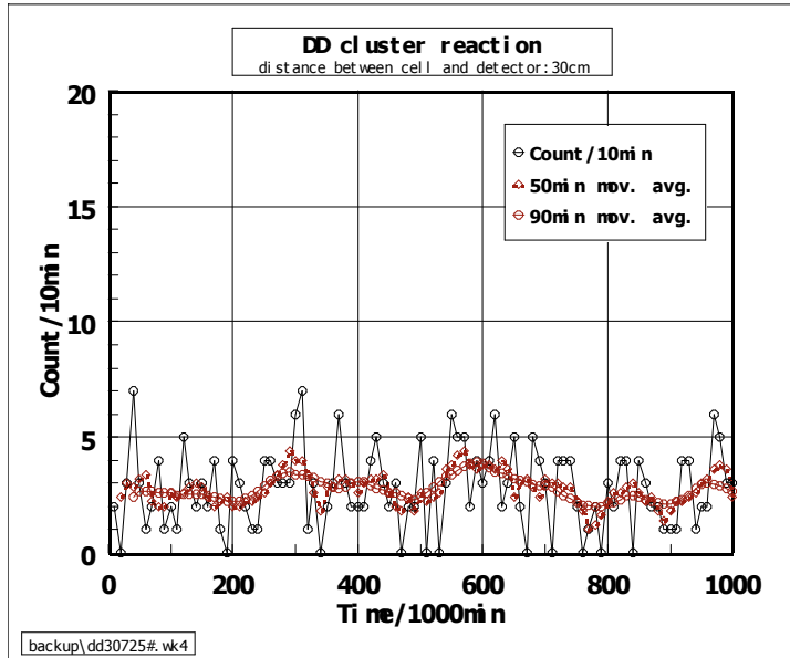
Fig.11: Rate of neutron count in 10min, 3 atm. D 2 gas, 8kG but room temperature.
