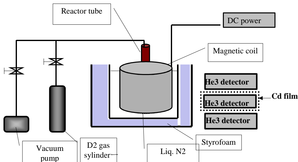
Fig.5: Schematic representation of the D 2 gas experimental set up
