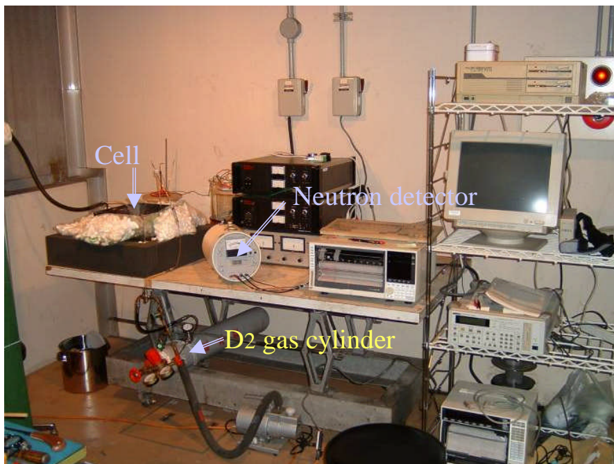
Fig. 4: Photo of D 2 gas experimental setup
