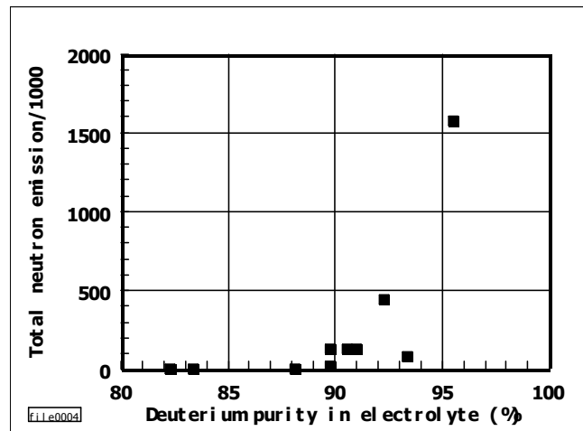
Fig. 3: Dependence of neutron on purity of D_2O
