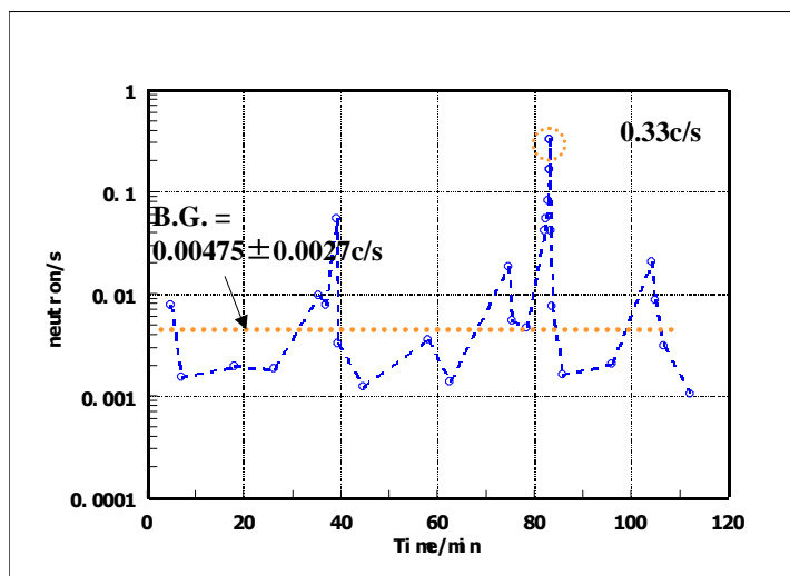
Fig.10: Real time representation of fig9.
