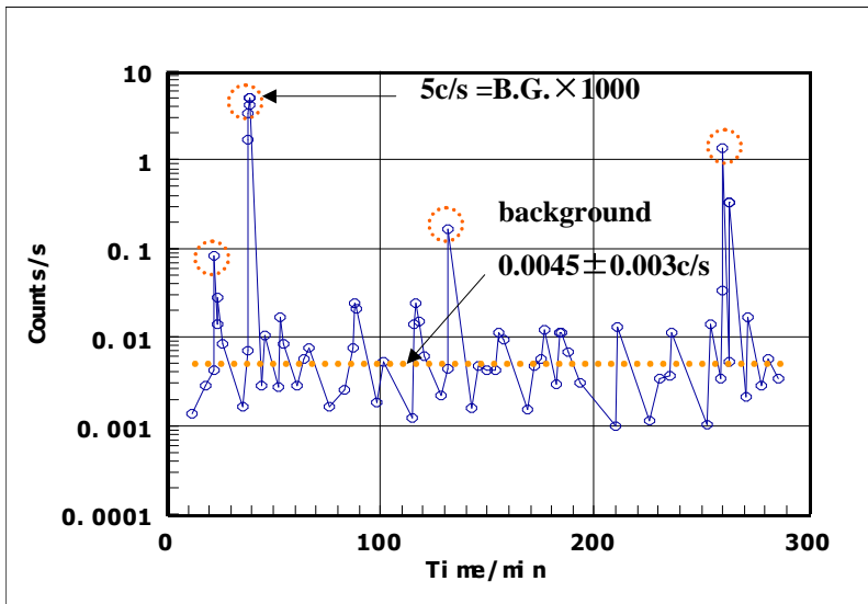
Fig.7: Real time representation of fig6
