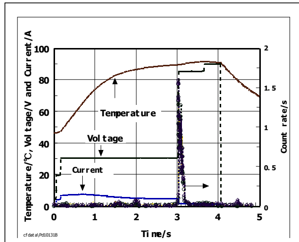
Fig. 2: neutron burst
