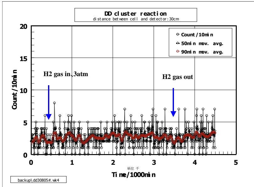
Fig.8: A case of H 2 gas at liquid N 2 temperature under 8kG.
