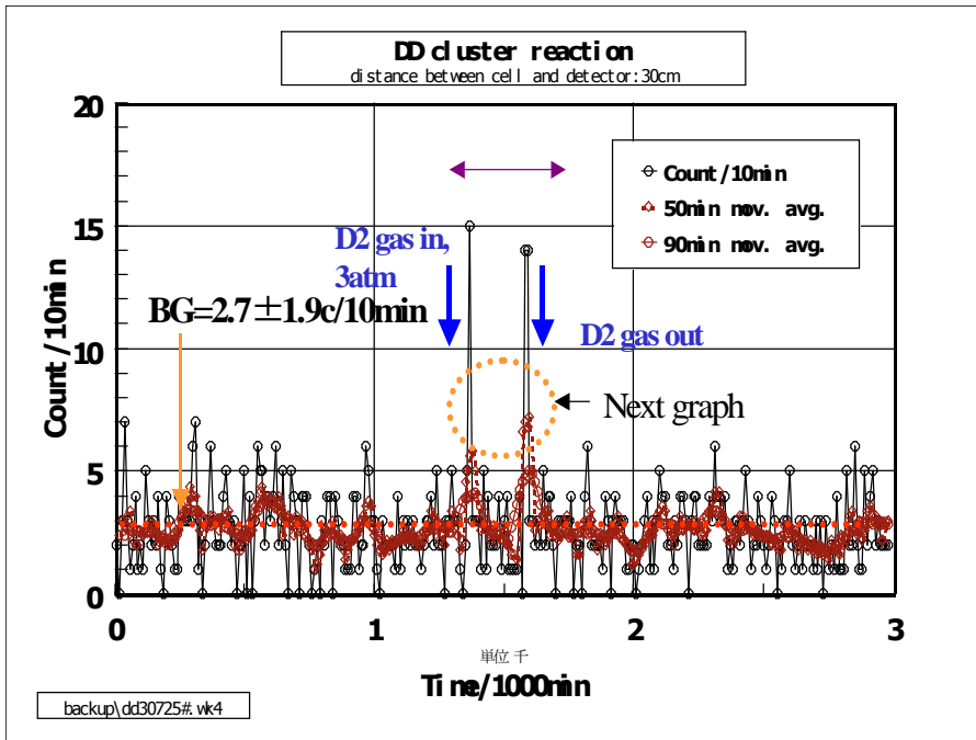
Fig.6: Typical rate of neutron count in 10min, 3 atm. D 2 gas, 8kG
