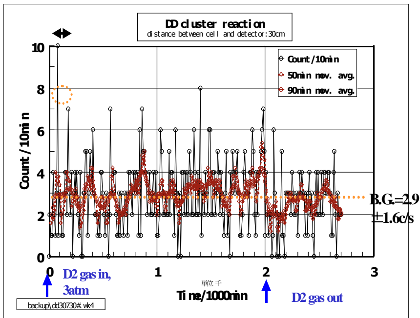
Fig.9: Rate of neutron count in 10min, 3 atm. D 2 gas, 8kG
