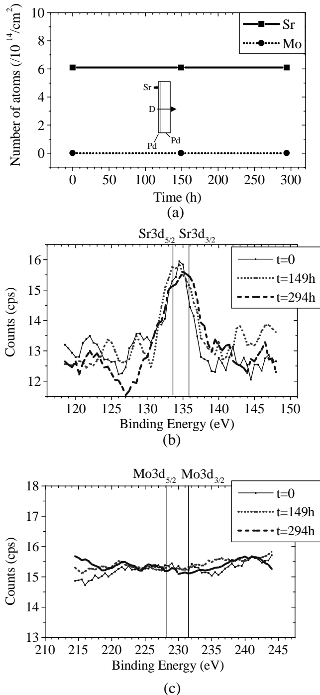
Fig. 8. Experimental results obtained by D 2 gas permeation through thin film and bulk Pd deposited with Sr: (a) Time variation in number of Sr and Mo atoms, (b) XPS spectrum of Sr, (c) XPS spectrum of Mo.
