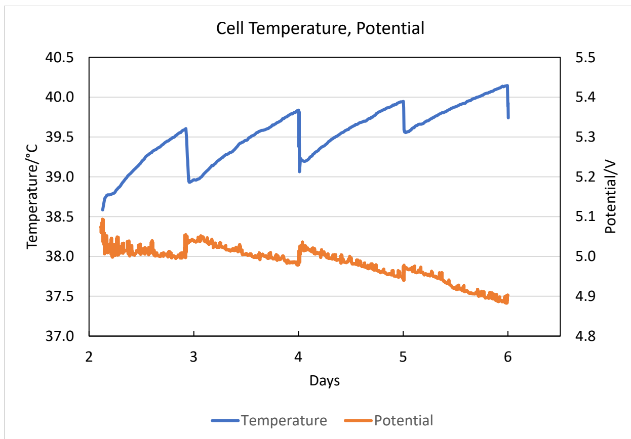
FIG. 1. Cell temperature (upper) and cell potential (lower) vs. time since cell was started for the electrolysis of D_2O in 0.6M Li_2SO_4 solution at pH 10 at a palladium rod cathode ( 0.4 \times 1.25 cm). The cell current was 400 mA, the water bath temperature was 30.00^\circ C , and the room temperature was 21^\circ C . The rate of excess enthalpy generation at the end of each day was 0.045 W (day 3), 0.066 W (day 4), 0.086 W (day 5), and 0.115 W (day 6). The accumulation of excess enthalpy for this period was on the order of 26 KJ. 3
