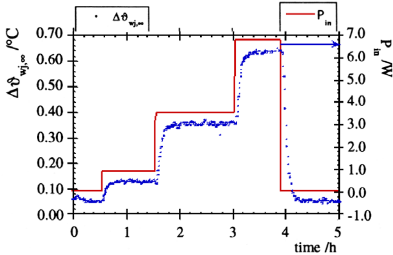
Fig. 1. Response of the cell at step variations of input power generated by the internal heater while electrolysis is running.
