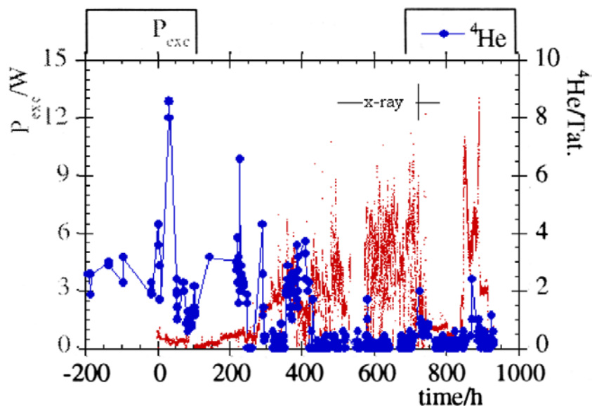
Fig. 3. Excess heat power (left scale) and 4 He (right scale) in an experiment with bundle-type cathode (250 μm dia. wires)
