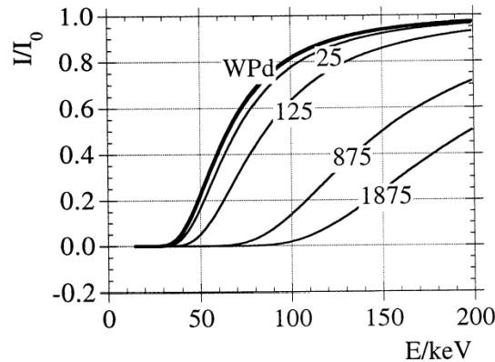
Fig. 7. Attenuation I/I_0 vs photon energy of Pd and materials between cathode and film (WPd=Without Pd) at different thickness (in \mu\text{m} ) of Pd crossed.
