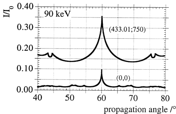
Fig. 9 Calculated transmission at 90 keV with two different positions of the source in the cathode
