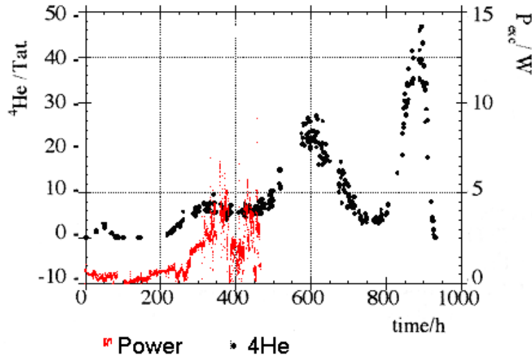
Fig. 4. Calculated {}^4\text{He} (left scale) and heat power excess (right scale)
