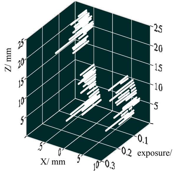
Fig. 6. Microdensitometry of the x-ray film placed parallel to the X,Z plane. Exposure is given in Roentgen (R)
