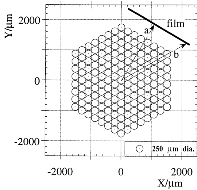
Fig. 8. Representation of the cross-section of an ideal bundle-type cathode with 169 wires of 250 \mu\text{m} dia. The cathodes used were made of 150 wires.
