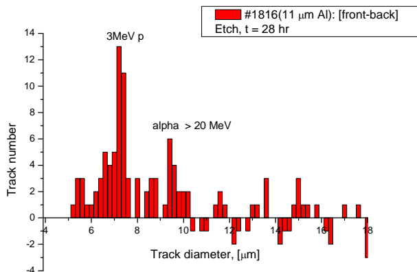
Figure 11 (a-d). Differential spectra (with subtracting of the background (the rear detector’s face tracks) of #1816 CR-39 detector (exposed during e-beam irradiation of 6 Pd/PdO:Dx samples during 1000 min) after its etching during 7 (a), 14(b), 21(c) and 28(d) hours. The shift of the “peaks” in a larger track diameter side with increase in etching time is well seen.
