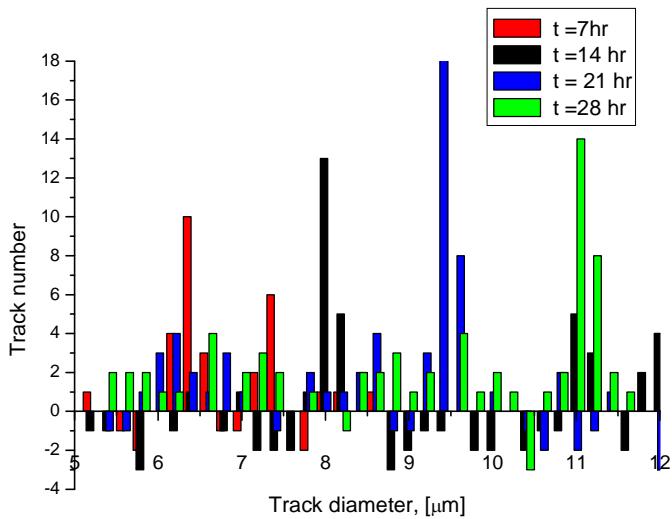
Figure 14. Shift in a main peak track diameter (1.4 MeV protons) following by sequential etching of #1816 detector covered with 25 micrometers thick Cu foil
