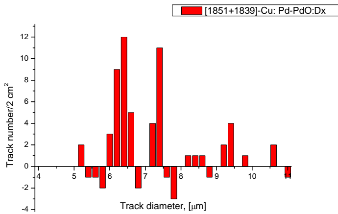
Figure 9. a. Differential spectra of the 25 \mu\text{m} Cu covered CR-39 detector (position 2 in Figure 2) obtained in the second series (20 runs) of experiments with the 6 Pd/PdODx samples. b. The sum obtained in both first (16 runs, Fig. 6b) and second (20 runs) series of experiments. Total time of 1+2 series is \tau = 1800 min, using 10 similar Pd/PdO:DX. The statistically significant bands of 1.4 MeV protons (track diameter in the range of 6.0-6.6 \mu\text{m} , consistent with the 3 MeV proton losses in 25 \mu\text{m} Cu foil) and 15 MeV alphas (track diameter near 7.4 \mu\text{m} , consistent with \sim 19 MeV alpha losses in 25 \mu\text{m} Cu foil) are appeared in the sum spectra (b).
