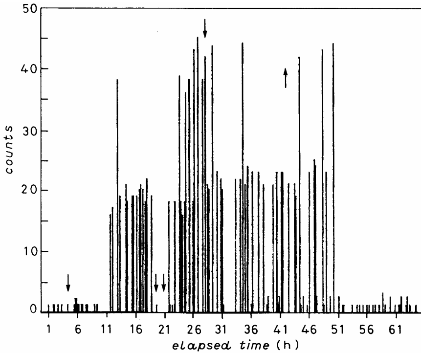
Fig. 8. Diagram showing the time evolution of the neutron emission counts (ordinate) during the first run (7-10 April, 1989) by De Ninno et al. [16]. The values indicated are integral counts over periods of 10 minutes.
