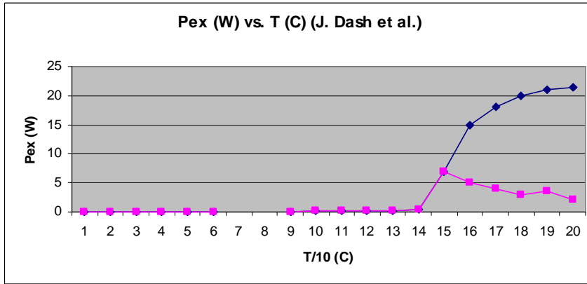
Fig. 5. Temperature dependence of the excess energy P_{ex} (W) from three experimental data sets obtained between June 20, 2006 and January 18, 2007. The high temperature region after bifurcation is an estimate, as explained in the text.
