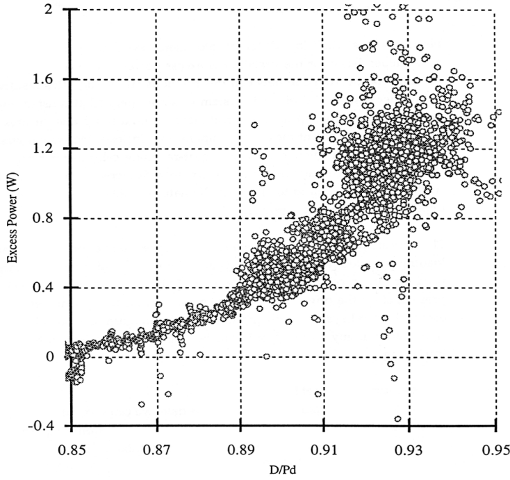
Fig. 6. Variation of excess power with loading ratio D/Pd obtained by McKubre et al. [9].
