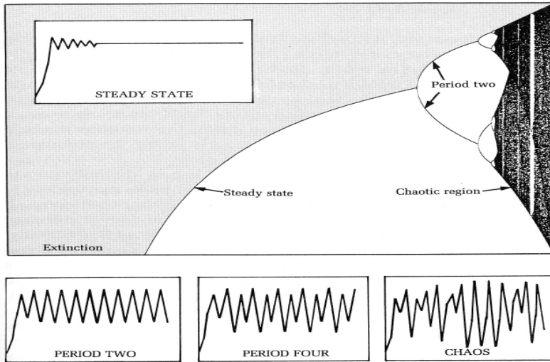
Fig. 7. Bifurcation diagram to show period-doubling and chaos (From “Chaos” by J. Gleick [15]. p.71). The main figure depicts x_\infty (ordinate, x_n at n = \infty ) vs. the parameter \lambda (abscissa) of the logistic difference equation, i.e. l.d.e., x_{n+1} = \lambda x_n(1 - x_n) ( 0 < x_0 < 1 ). The inserted figures, a) Steady state, b) Period two, c) period four, and d) chaos, depict variations of x_n with increase of suffix n (temporal variation if n increases with time) for four values of \lambda ; a) 1 < \lambda < 3 , b) 3 < \lambda < 3.4 , c) \lambda \approx 3.7 , d) 4 < \lambda . The region a), b) and d) correspond to “Steady state”, “Period two” and “Chaotic region” in the main figure, respectively.
