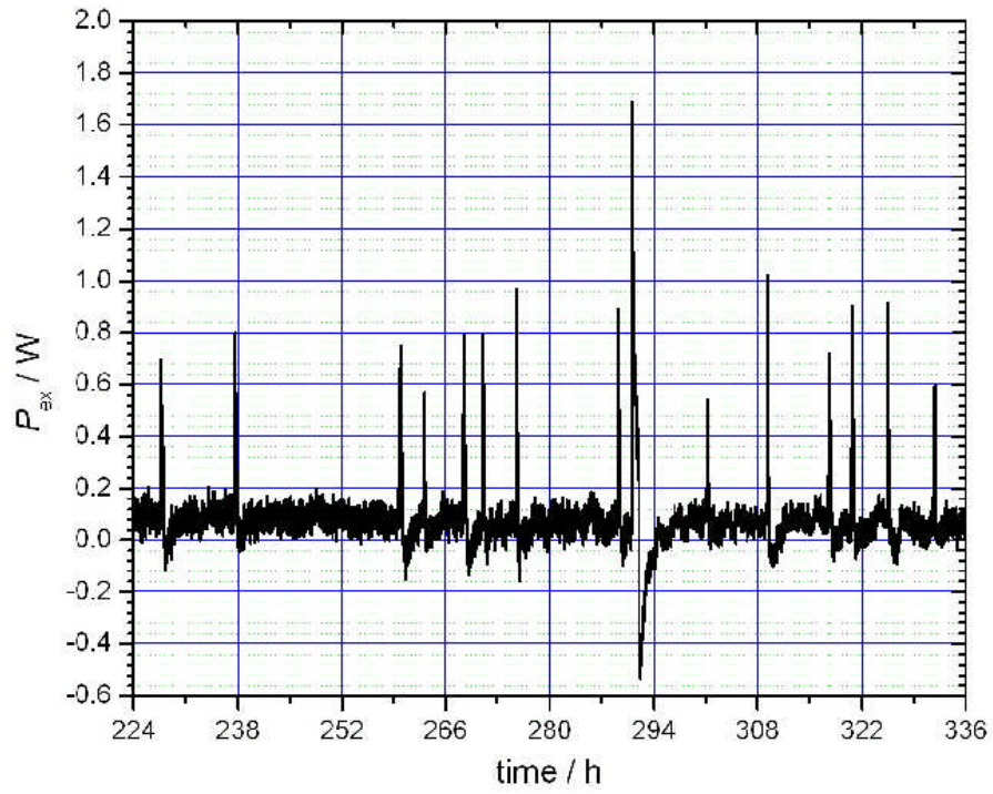
Fig. 2. Excess power pulses and bursts during a 112 hour period of an experiment (061026) which lasted 14 days as a whole.
