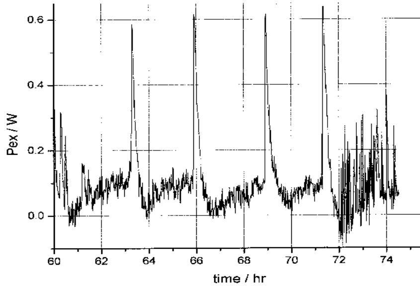
Fig. 3. Excess power pulses during a 14 hour period of an experiment (070108) which lasted 12 days as a whole.
