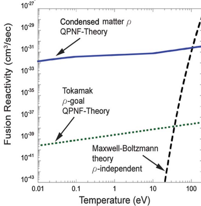
Fig. 1. Fusion reactivity, \langle \sigma v \rangle , of D(d,p)^3H reaction in units of \text{cm}^3/\text{sec} as a function of temperature kT in units of eV. The dashed line, the solid line, and the dotted line corresponds the results calculated using the MB distribution, the GY distribution with \rho = 10^{22}\text{cm}^{-3} , and the GY distribution with \rho = 10^{15}\text{cm}^{-3} , respectively.
