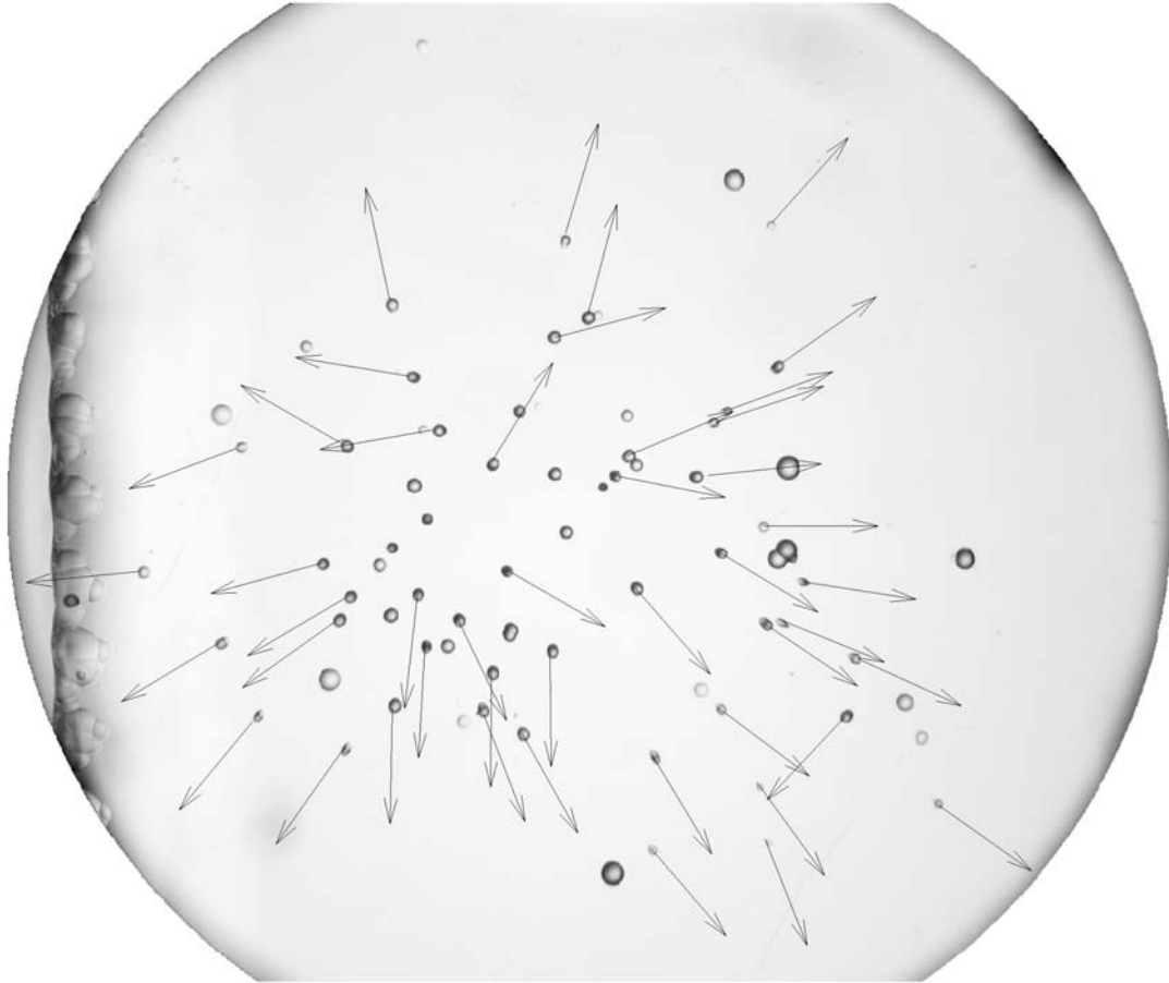
Figure 3. Shower of etch pits on a detector chip supported in air under a nickel cathode. The width of the image is approximately 2mm. Arrows indicate the directions in which charged particles impinged on the chip. The electrolyte was \text{Li}_2\text{SO}_4 in \text{H}_2\text{O} . (The virgin chip was etched before beginning the experiment to reveal pre-existing particle tracks. During the following etch they grew to twice the diameter of the experimental pits and can be distinguished by their large size.)
