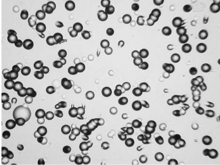
Figure 1. Etch pits on the surface of a CR-39 plastic detector chip suspended in the vapor over an active electrolysis cell. Each pit marks the location of a track of damaged material where a charged particle has penetrated the chip. A roughly conical pit has developed during etching because the etchant attacks the damaged material of the track more rapidly than it attacks the adjacent undamaged material. The area shown measures approximately 0.58mm x 0.44mm. The mean diameters of the darker circular pits are approximately 24 microns.
