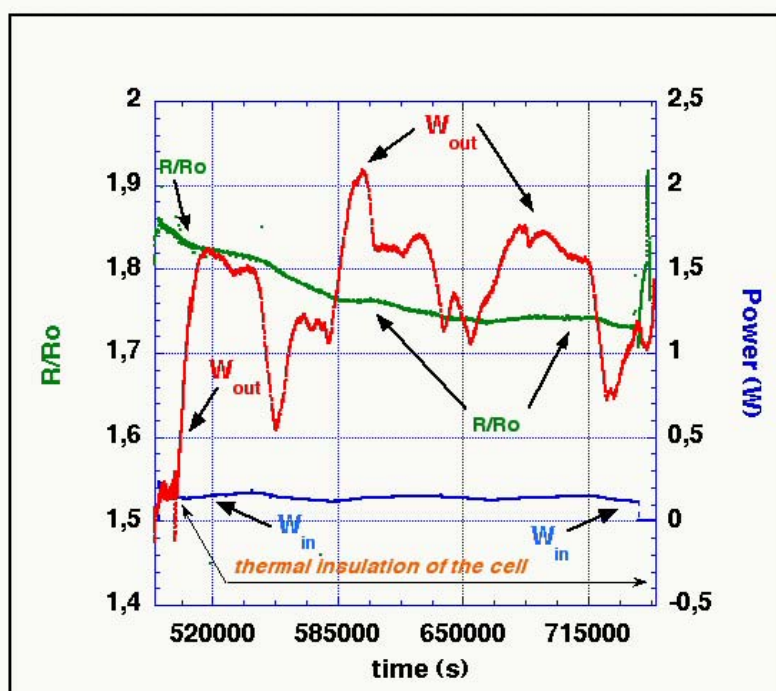
Figure 5 – Flow calorimeter measurements. W_{in} is the total power input. W_{out} is the power flowing out of the calorimeter with the outgoing water flow.
