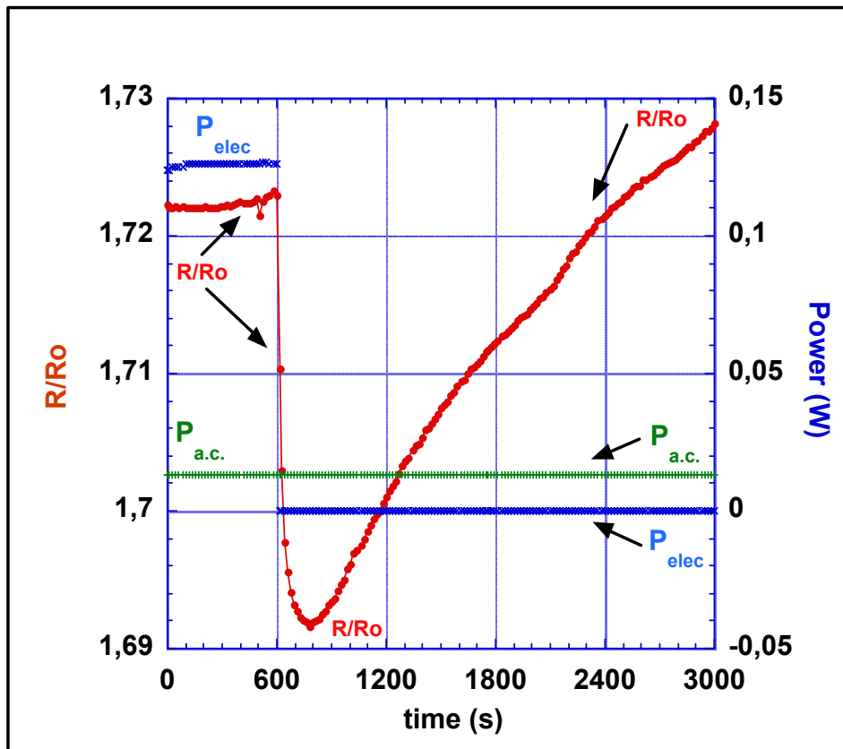
Figure 2 – The fall in cathode resistance when the electrolysis is switched off. R/Ro is the ratio between the actual resistance R and resistance at D/Pd=0. P elec is the power input due to the electrolysis current. P a.c. is the power input due to the a. c. current used to measure the cathode resistance.
