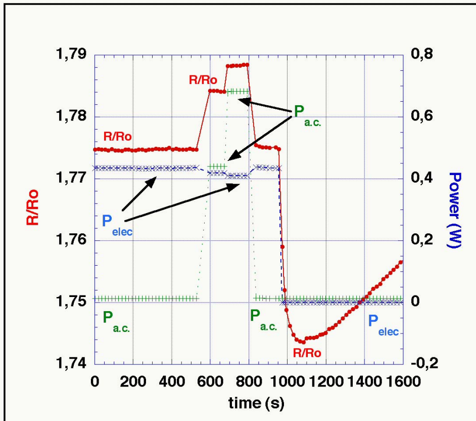
Figure 4 – Self calibration procedure. On the left side it is shown the increase of R/R_o due to the Joule effect produced by increasing the a. c. power input ( P_{a.c.} ). On the right side it is shown the R/R_o drop down when the electrolysis power ( P_{elec} ) is reduced.
